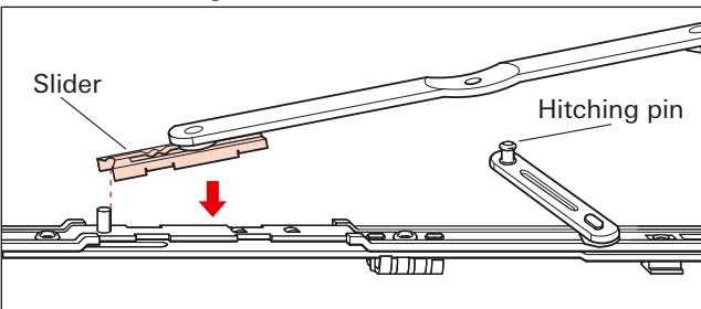
Standard tilt-range (140mm)
