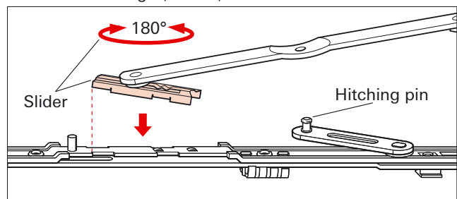
Reduced tilt-range (80mm)
